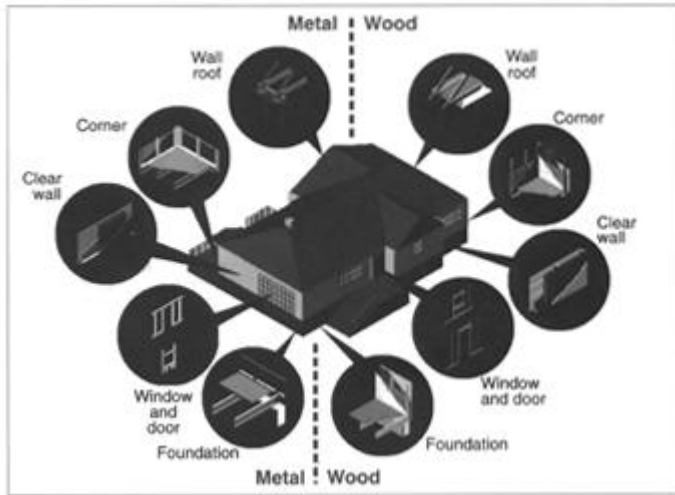
Figure 1. Interface details for metal and wood framing.
